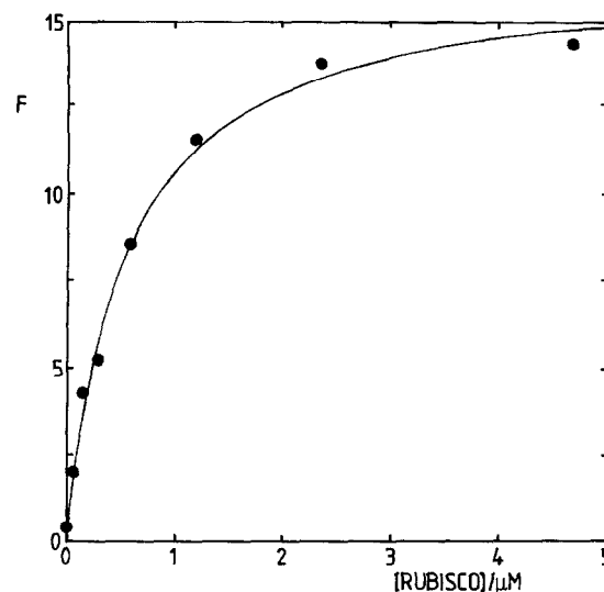
Fig. 3. Fluorescence, F , of RH421 in arbitrary units as a function of the rubisco concentration at a constant total dye concentration of 408 nM; \lambda_{\text{ex}} = 500 nm (+GG475 cut-off filter), \lambda_{\text{em}} = 640 nm, bandwidths = 3 nm, T = 25^\circ\text{C} . The solid line represents a fit of the data to Eq. 4.
