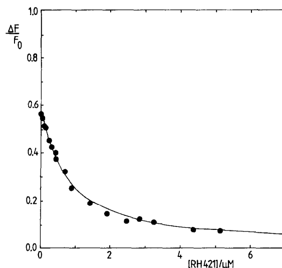
Fig. 4. Variation of the relative fluorescence change, \Delta F / F_0 , of RH421 after the addition of 0.53 mM MgATP in the presence of \text{Na}^+, \text{K}^+ -ATPase membrane fragments from rabbit kidney as a function of the dye concentration; [Protein] = 29 \mu\text{g}/\text{ml} , \lambda_{\text{ex}} = 570 nm (+OG550 cut-off filter), \lambda_{\text{em}} = 650 nm (+RG630 cut-off filter), bandwidths = 5 nm, T = 20°C. F_0 refers to the fluorescence prior to the addition of ATP. The solid line represents a fit of the data to Eq. 11.
